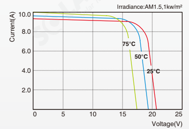
SLP160S-12 I-V Curves
