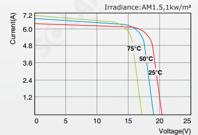
SLP100-12U I-V Curves
