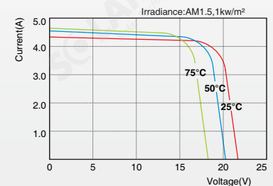
SLP070-12U I-V Curves
